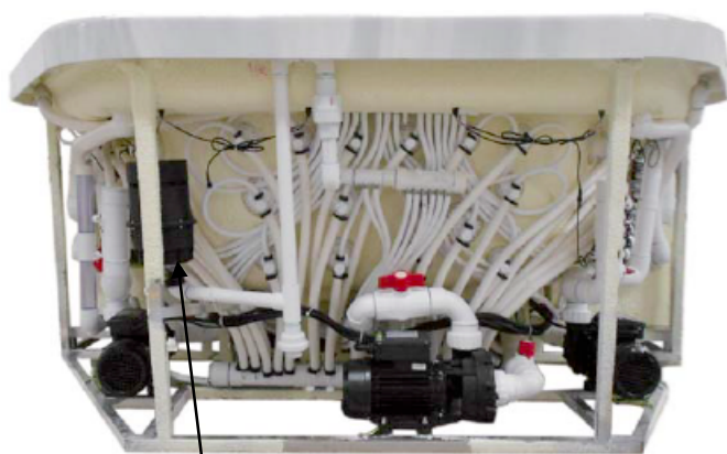
Blower
